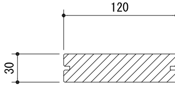
EP-LM1203断面図
